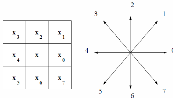
Fig. 6.2 The 8-neighborhood and the associated eight directions
